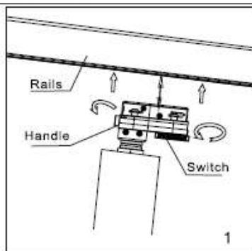
Rail mounted
