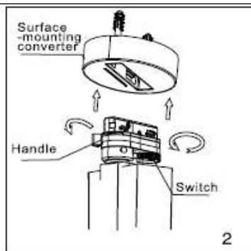
Surface-mounted
