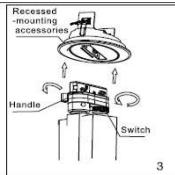
Recessed-mounted
